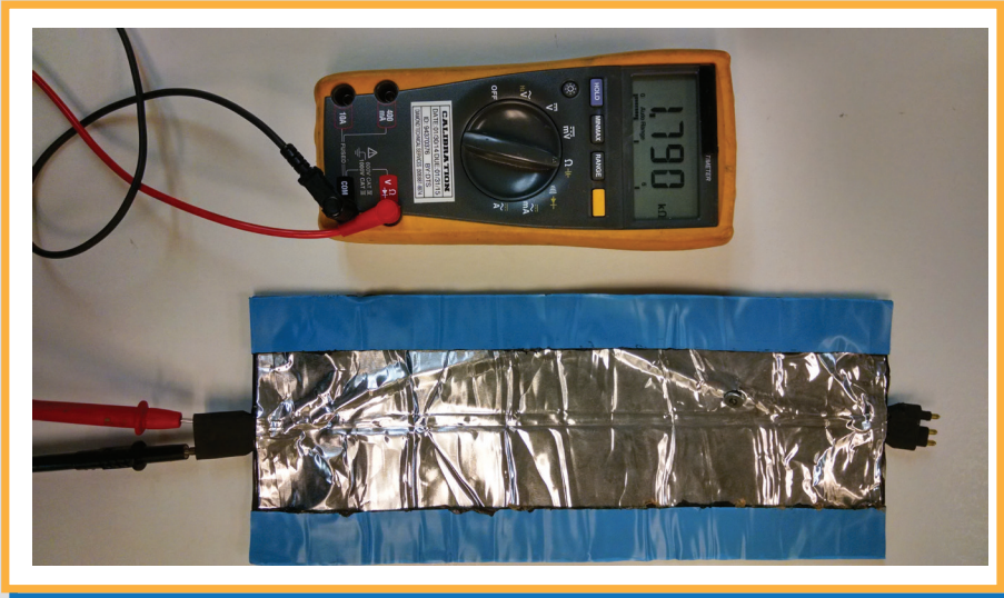
Figure 14. Checking Resistance
