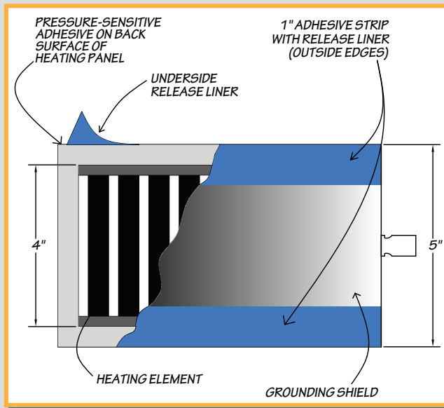
Figure 1. Heating Panel Construction
